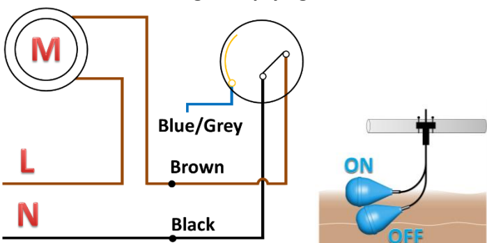
Fig.2 emptying
