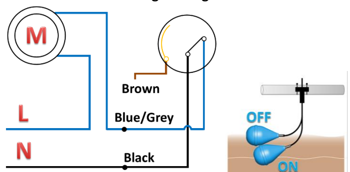
Fig.3 filling
