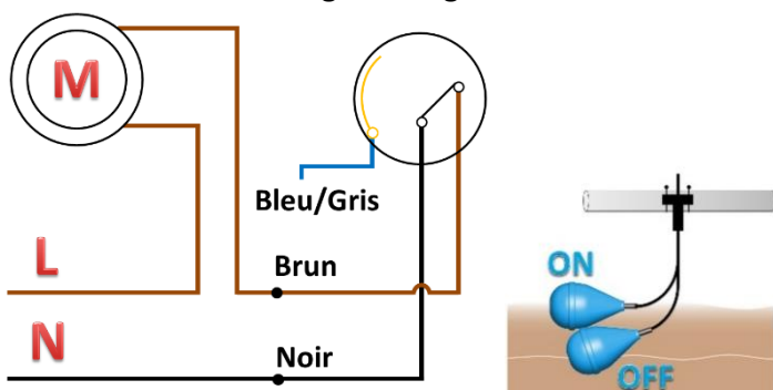
Fig.2 vidange
